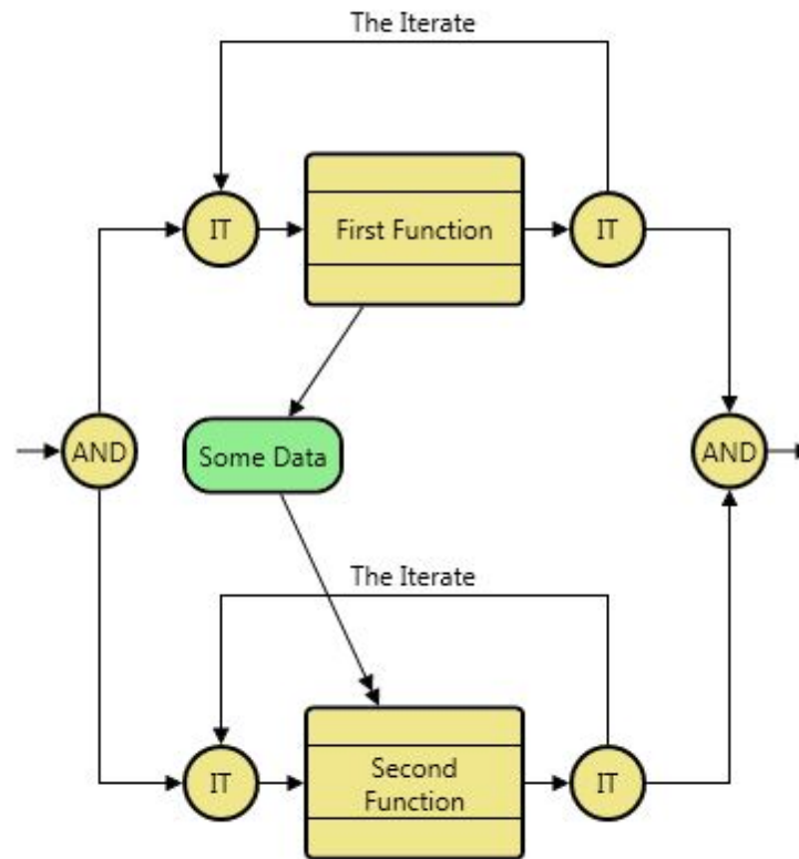
Figure 48 Link-Item Model
