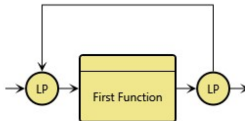
Figure 40 Loop Construct
