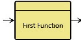
Figure 18 Single Function
