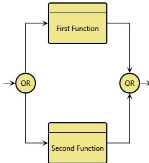
Figure 22 Select Construct
