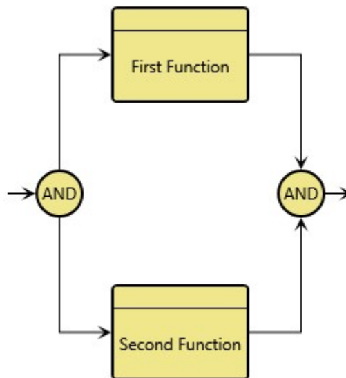
Figure 24 Parallel Construct
