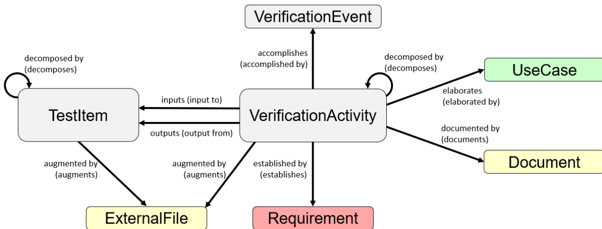
Figure 25 Test Planning
