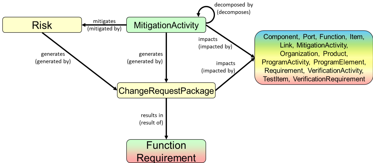
Figure 10 Mitigation Activities
