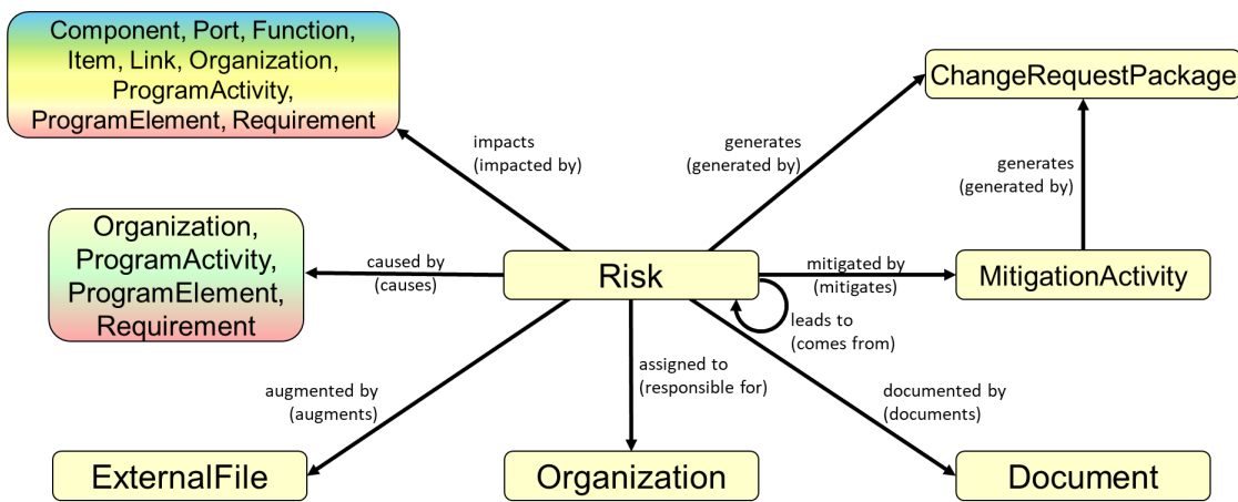
Figure 9 Risk Management
