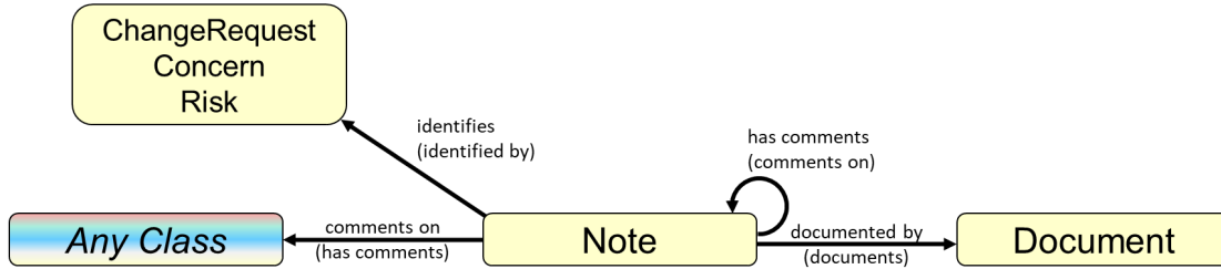
Figure 8 Note Class
