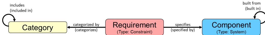
Figure 11 Constraint Requirements
