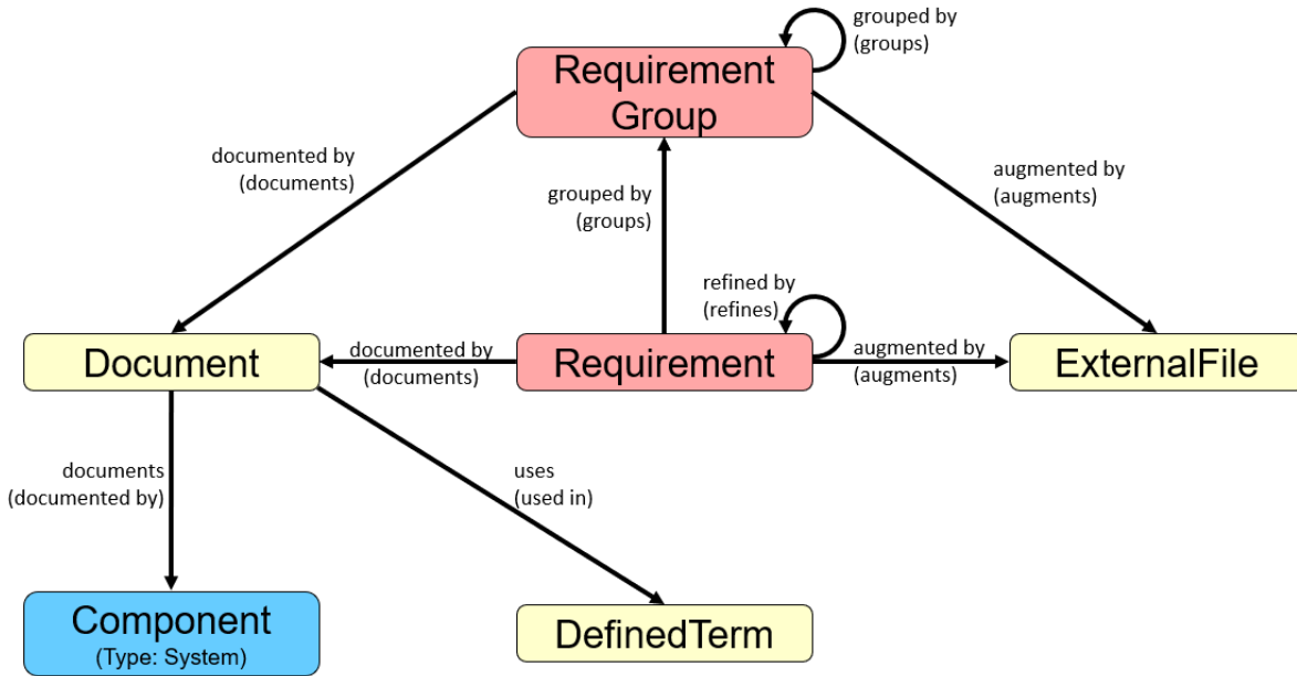
Figure 3 Source Requirements
