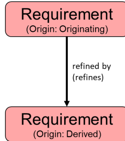
Figure 6 Derived Requirements
