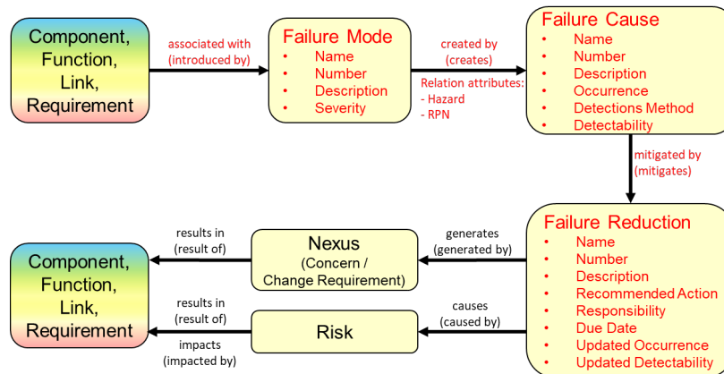
Figure 1. Overall FMEA Schema Extension
