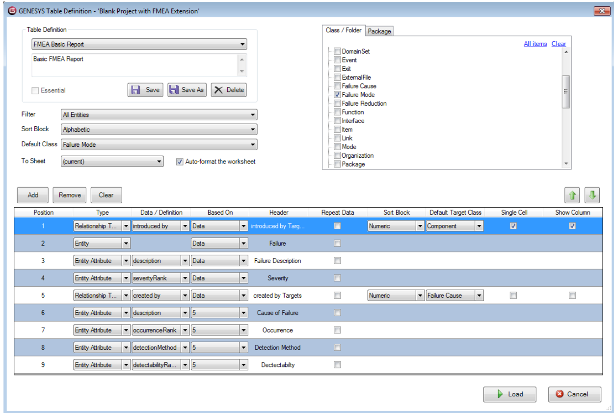
Figure 3 FMEA Basic Report
