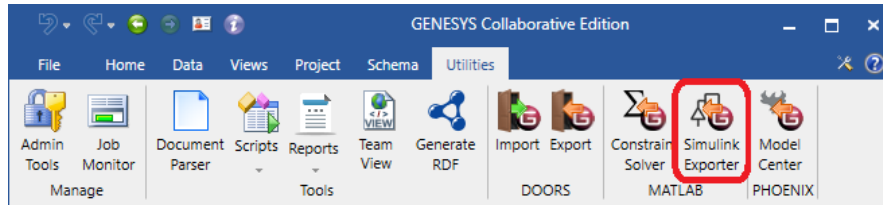
Figure 8. Simulink Exporter
