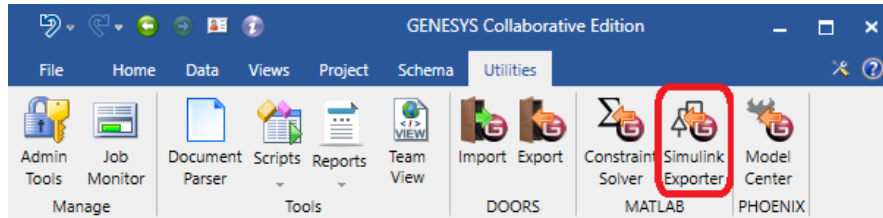
Figure 8. Simulink Exporter
