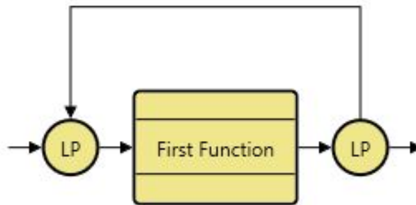
Figure 42 Loop Construct
