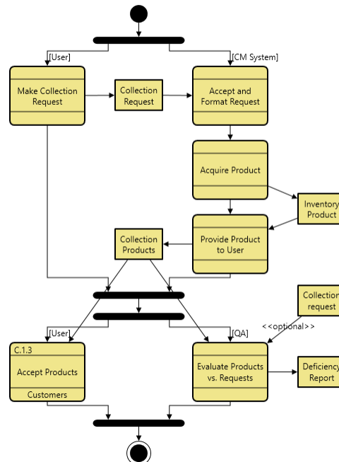
Figure 17 Activity Diagram
