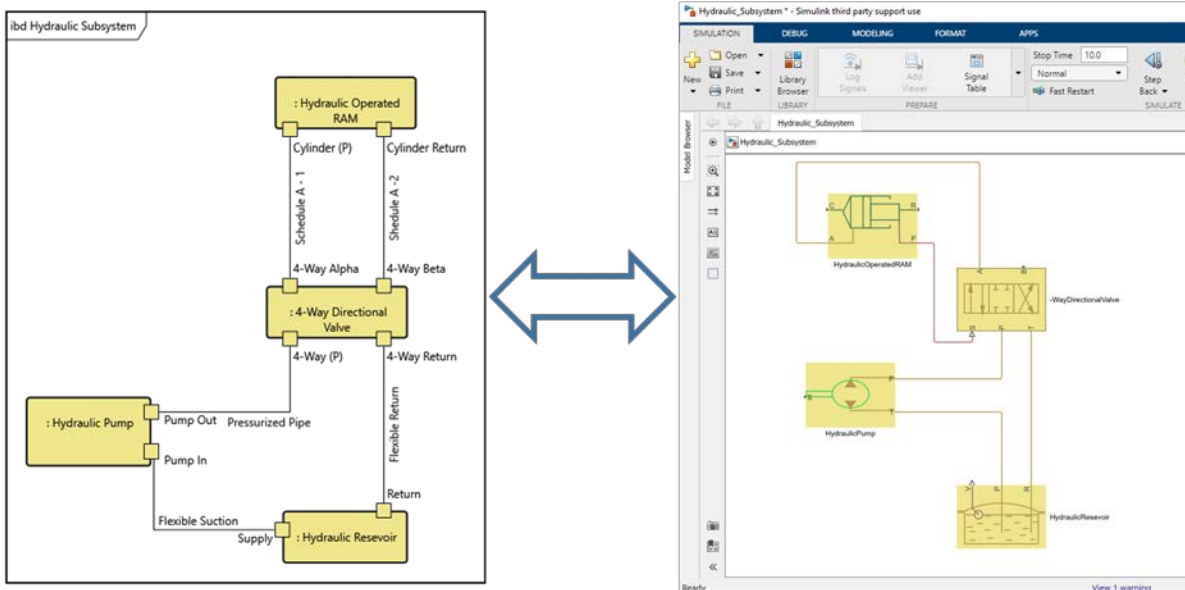
Figure 11. Two models: Simulink and GENESYS
