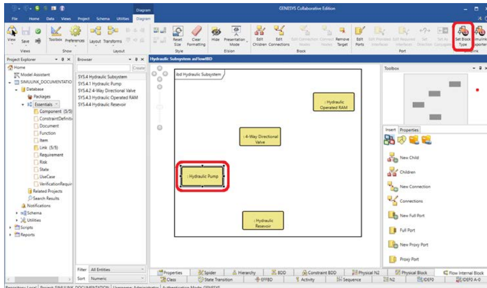
Figure 4. Flow IBD Setup to connect With Simulink
