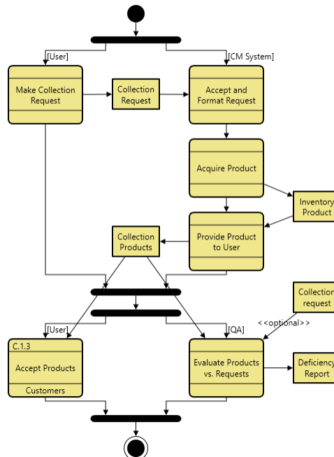
Figure 16 An Activity Diagram
