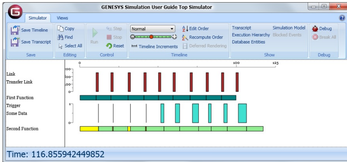
Figure 52 Simulation Results with Item Size = 1000.0, Link Capacity = 1000.0, Delay = 0.5
