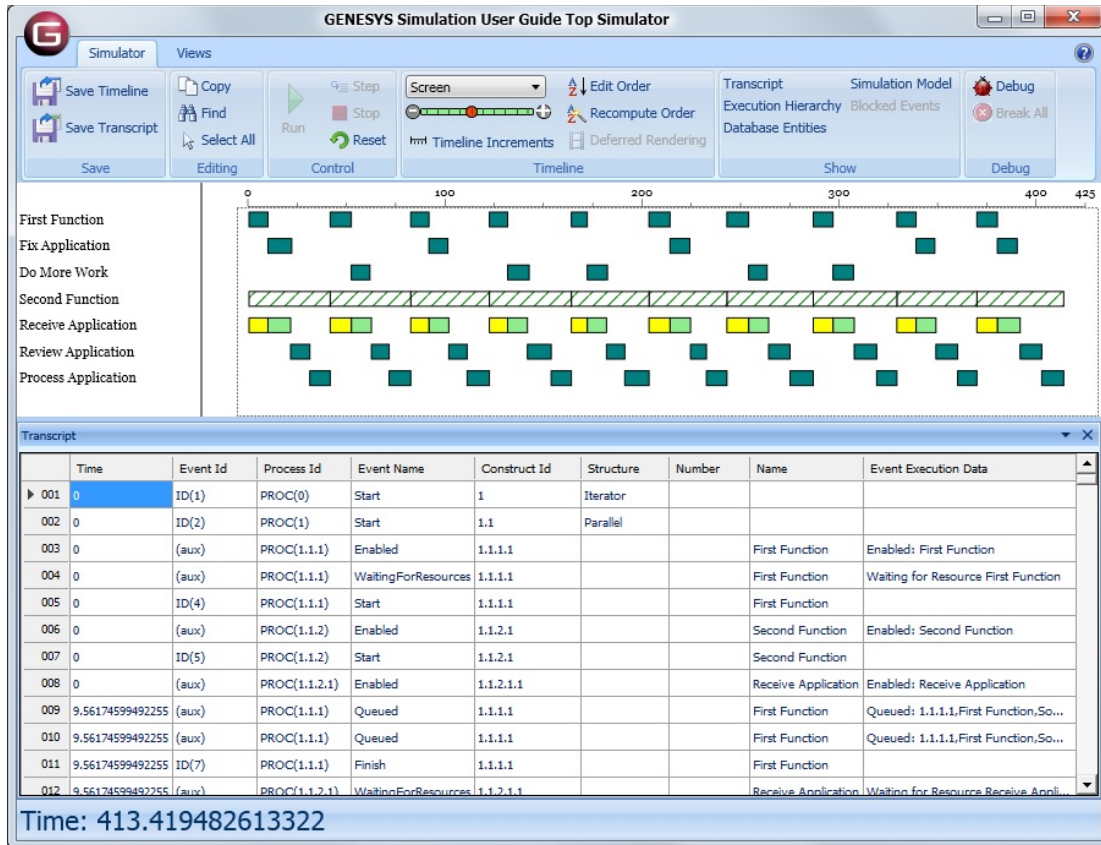
Figure 39 Results of Model Containing Decomposition
