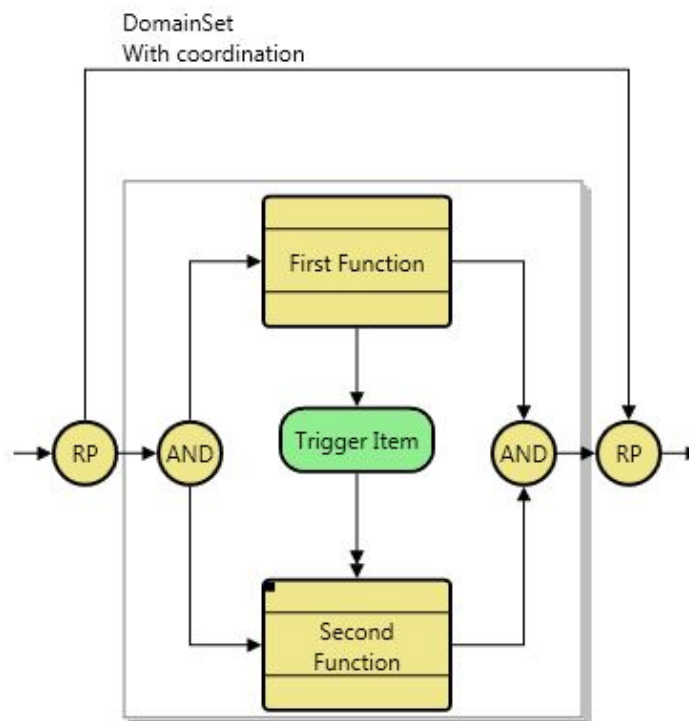
Figure 44 A Replicate Construct
