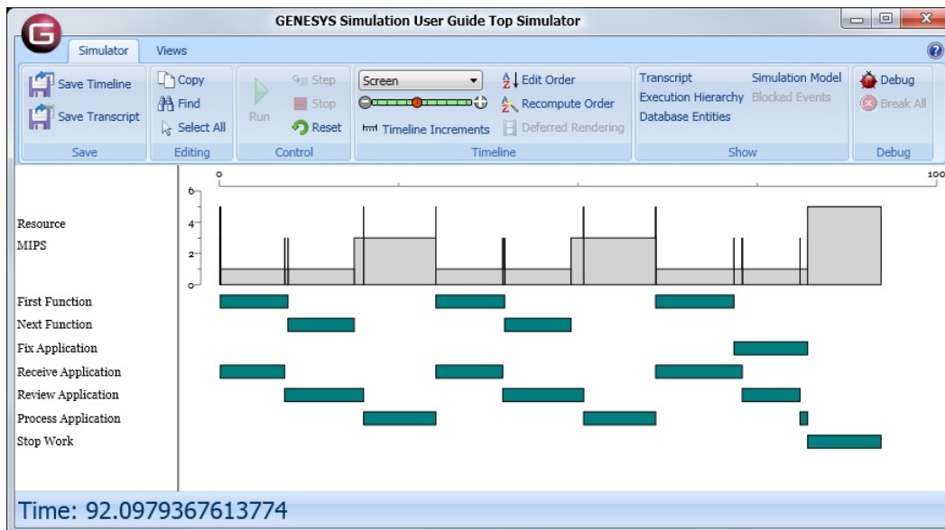
Figure 54 Loop Model with Adequate Resources
