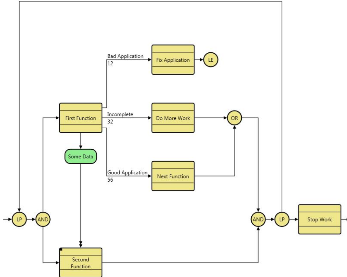
Figure 42 EFFBD with Loop and Loop Exit
