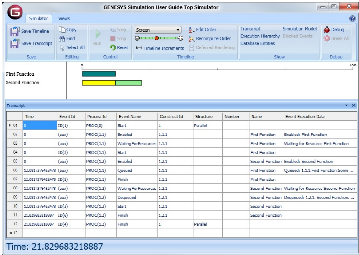
Figure 30 Trigger Item Simulation Results
