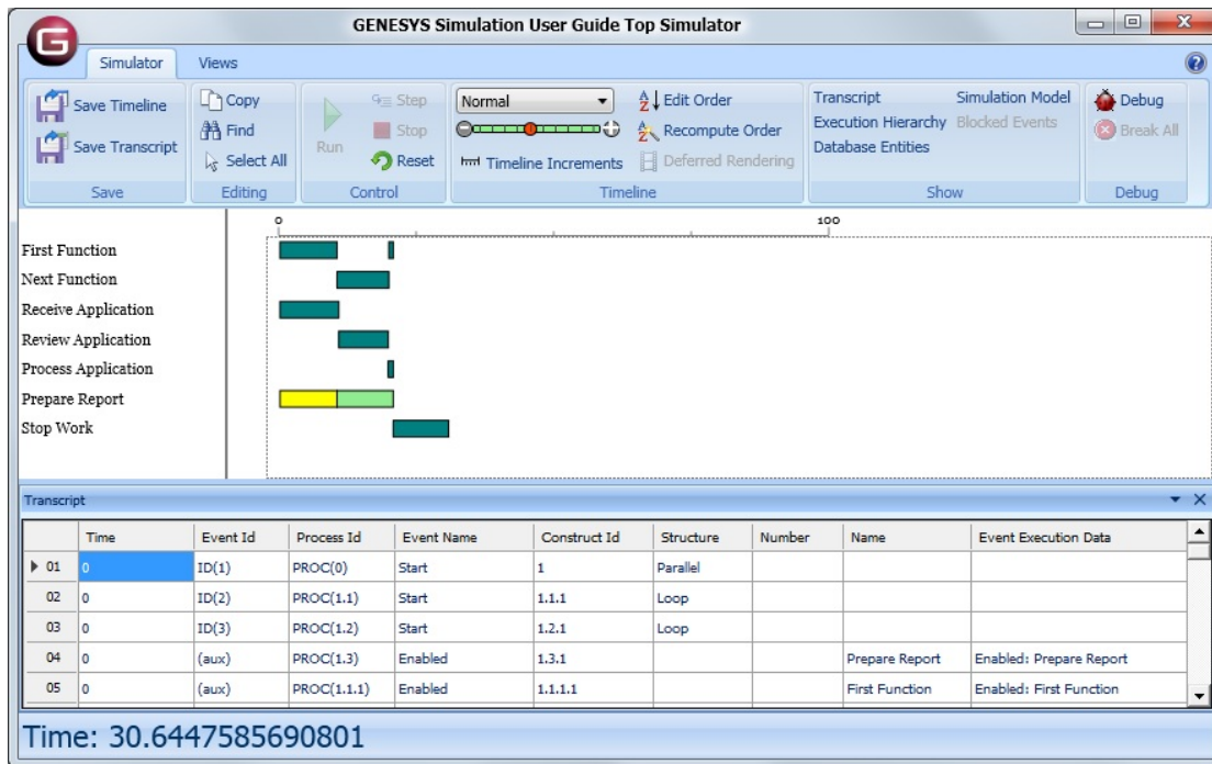
Figure 47 Simulation Results with Kill Branch
