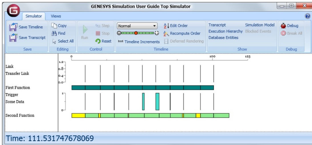
Figure 50 Simulation Results with Item Size = 0.0, Link Capacity = 1000.0, Delay = 0.0
