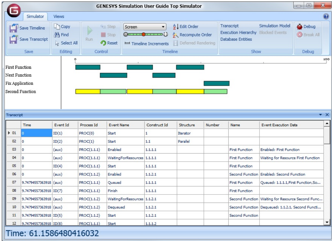
Figure 34 Multi-Exit Function Construct Simulation Results
