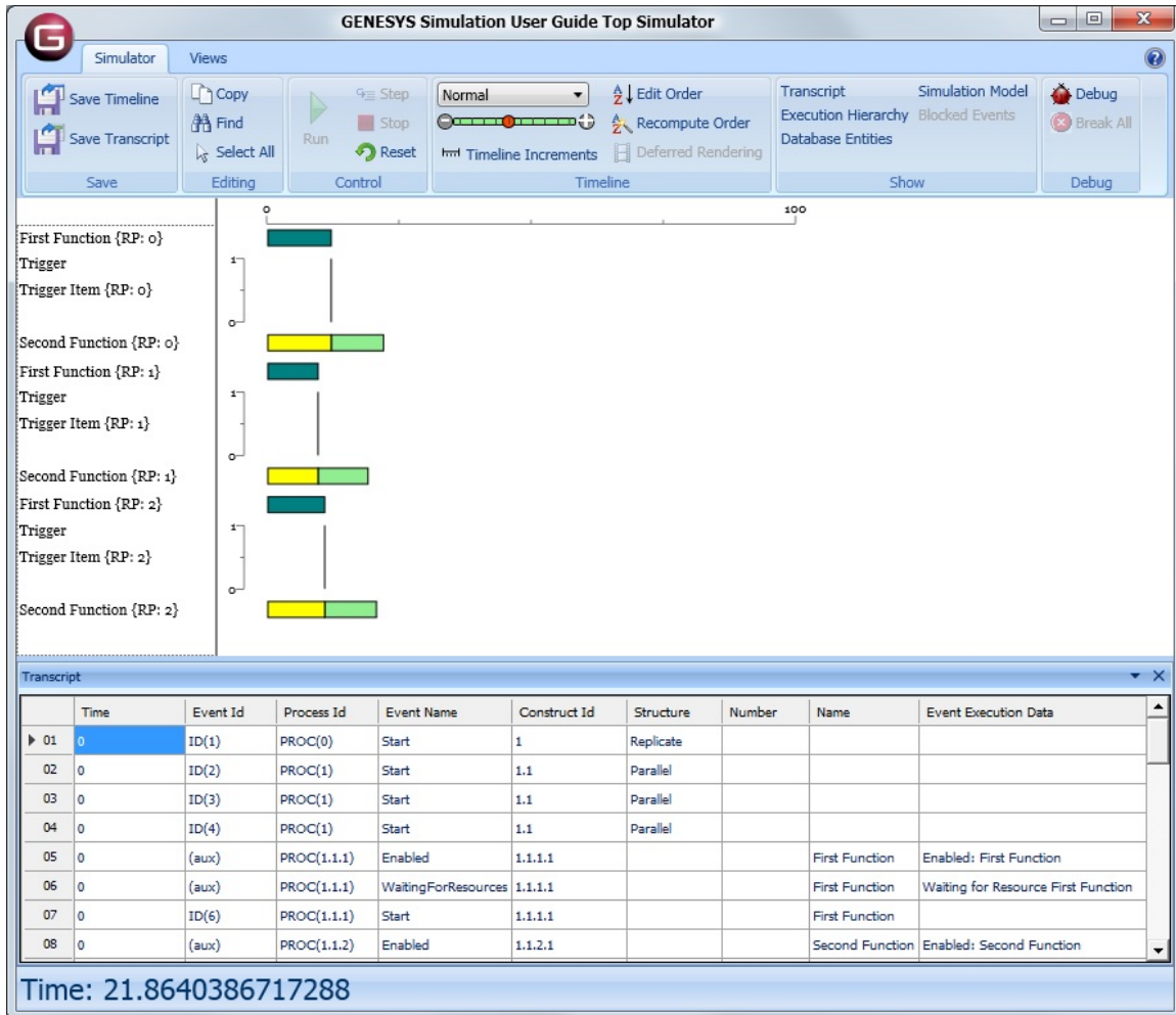
Figure 45 Results for Model with A Replicate Construct
