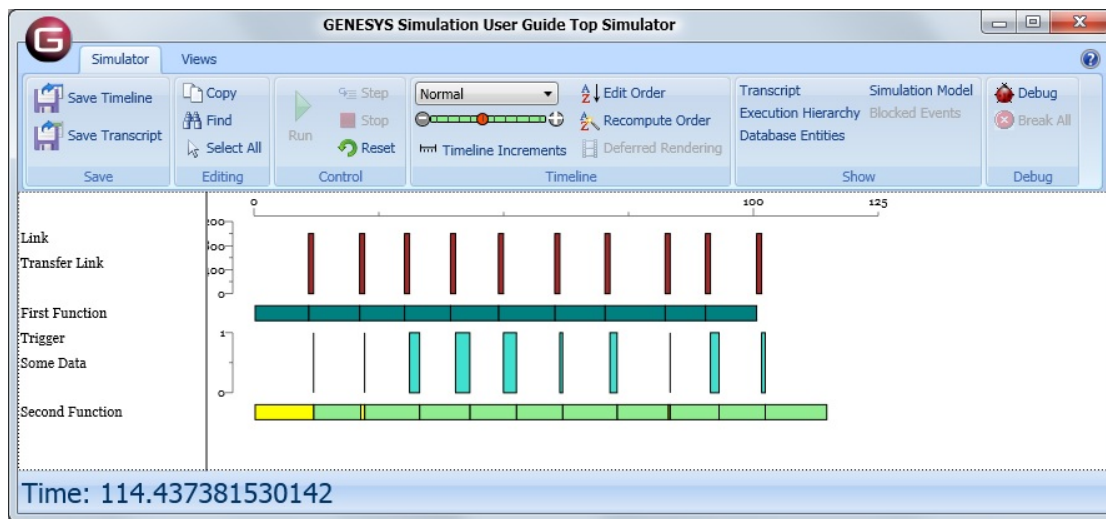
Figure 51 Simulation Results with Item Size = 1000.0, Link Capacity = 1000.0, Delay = 0.0
