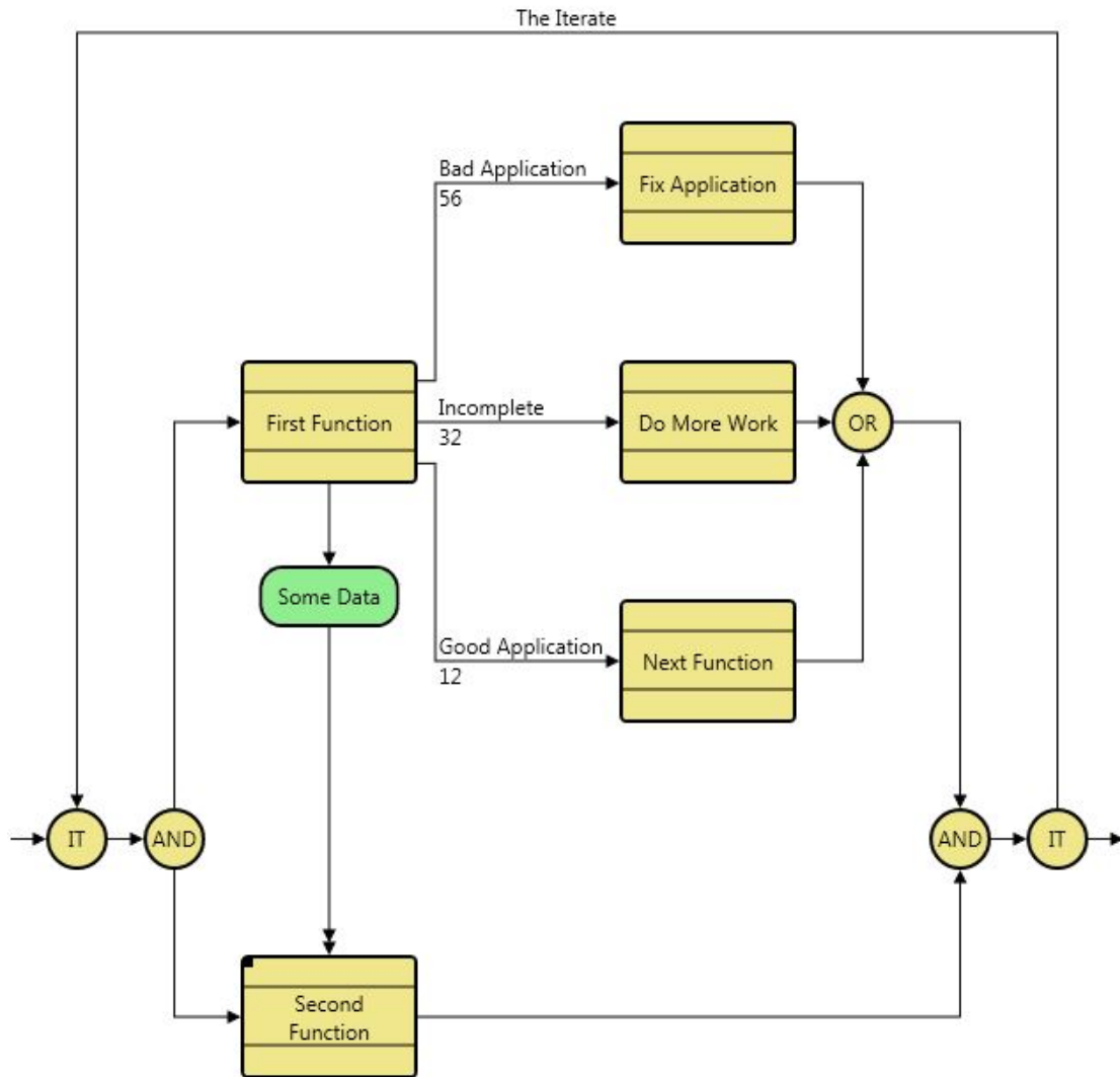
Figure 38 Model Containing Decomposition
