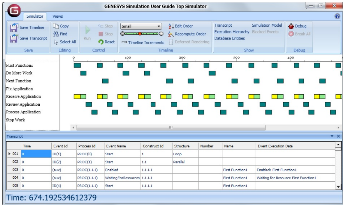
Figure 43 Results for Model with Loop and Loop Exit
