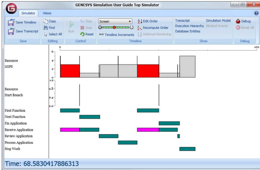
Figure 55 Loop Exit Model with Trigger-Type Resource
