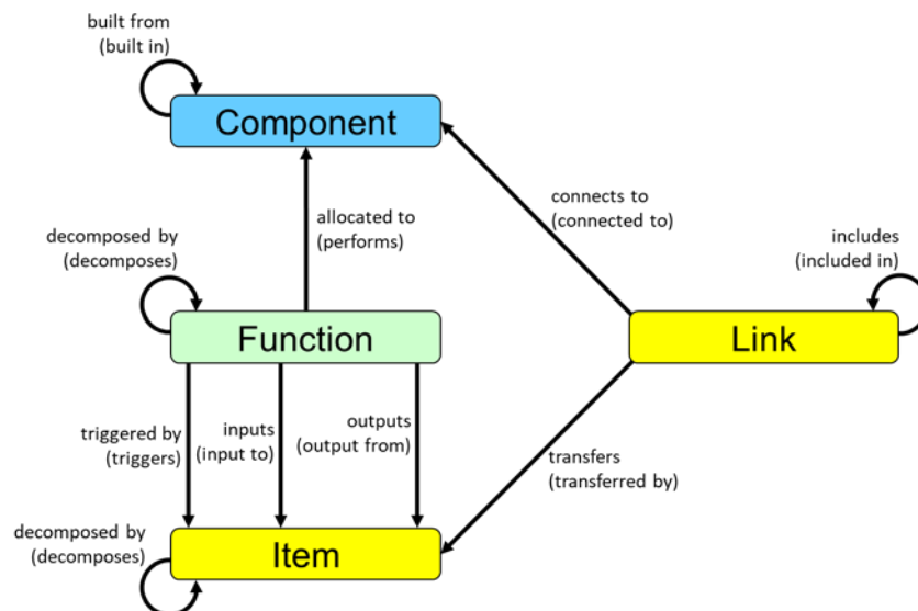
Figure 48 Link Schema Diagram
