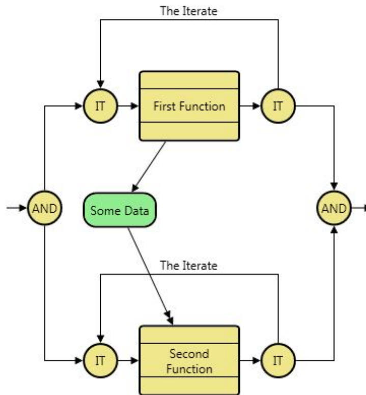
Figure 49 Link-Item Model
