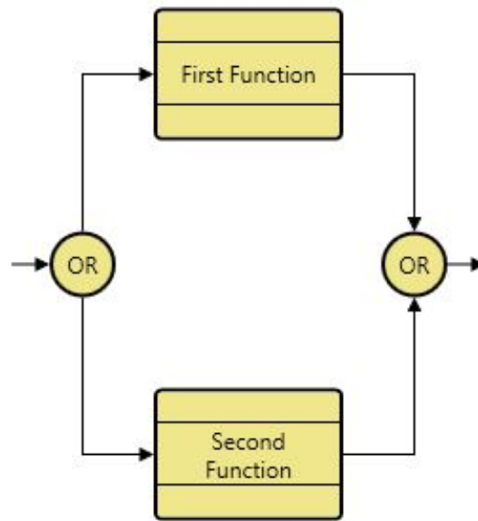
Figure 23 Select Construct
