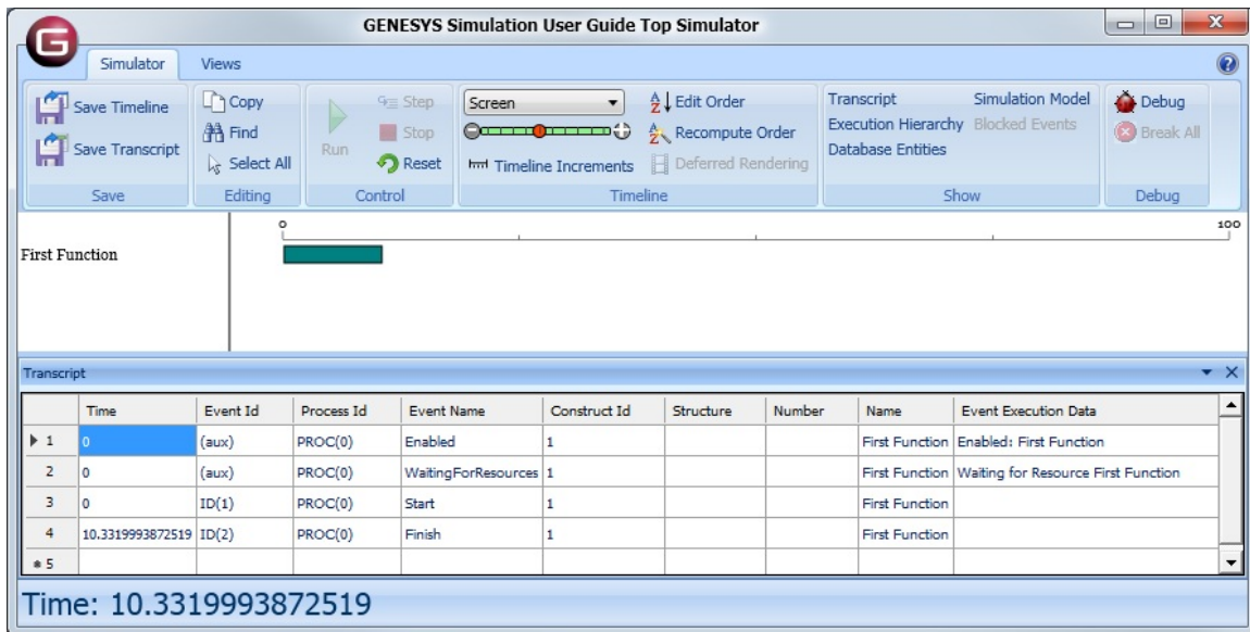
Figure 20 Single Function Simulation Results
