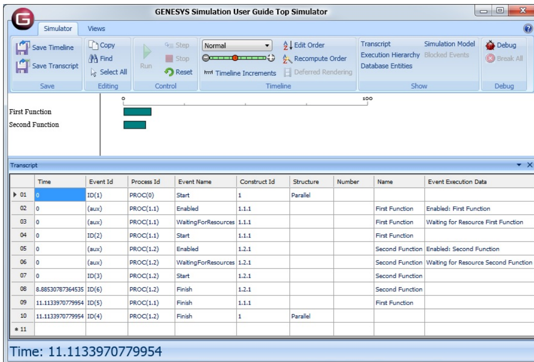
Figure 26 Parallel Construct Simulation Results
