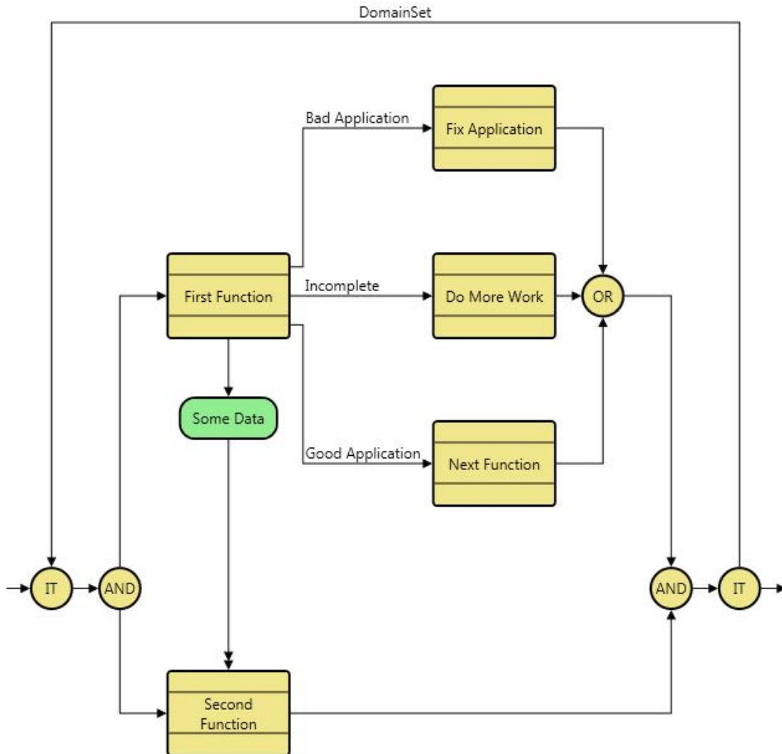
Figure 33 A Multi-Exit Function Construct
