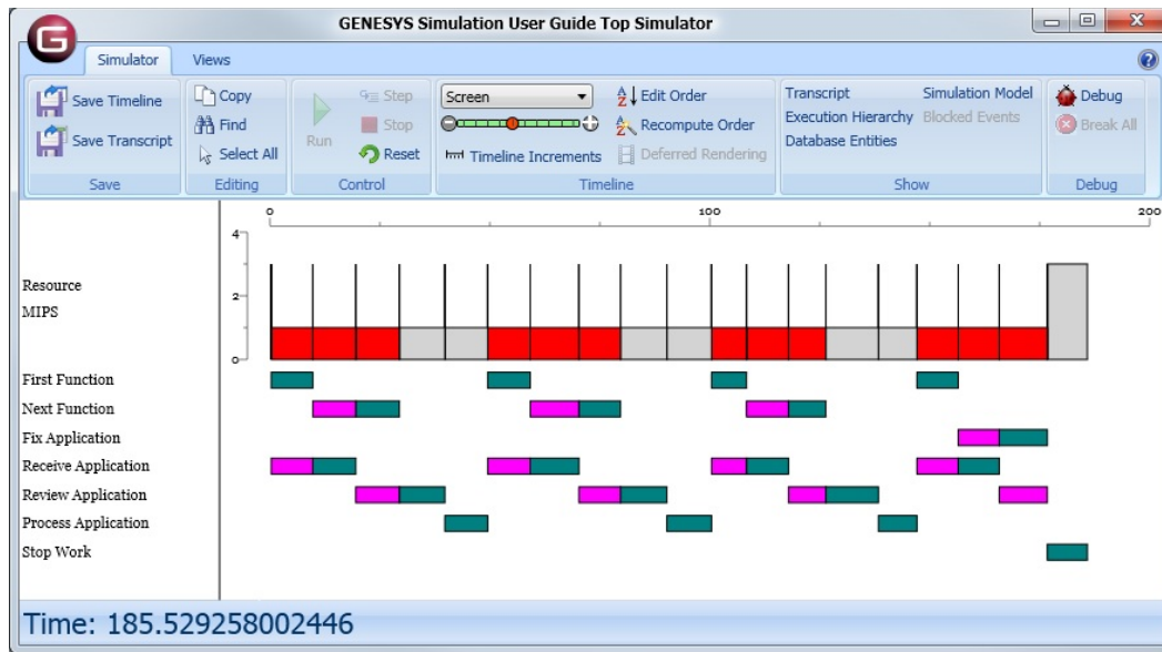
Figure 53 Loop Model with Insufficient Resources
