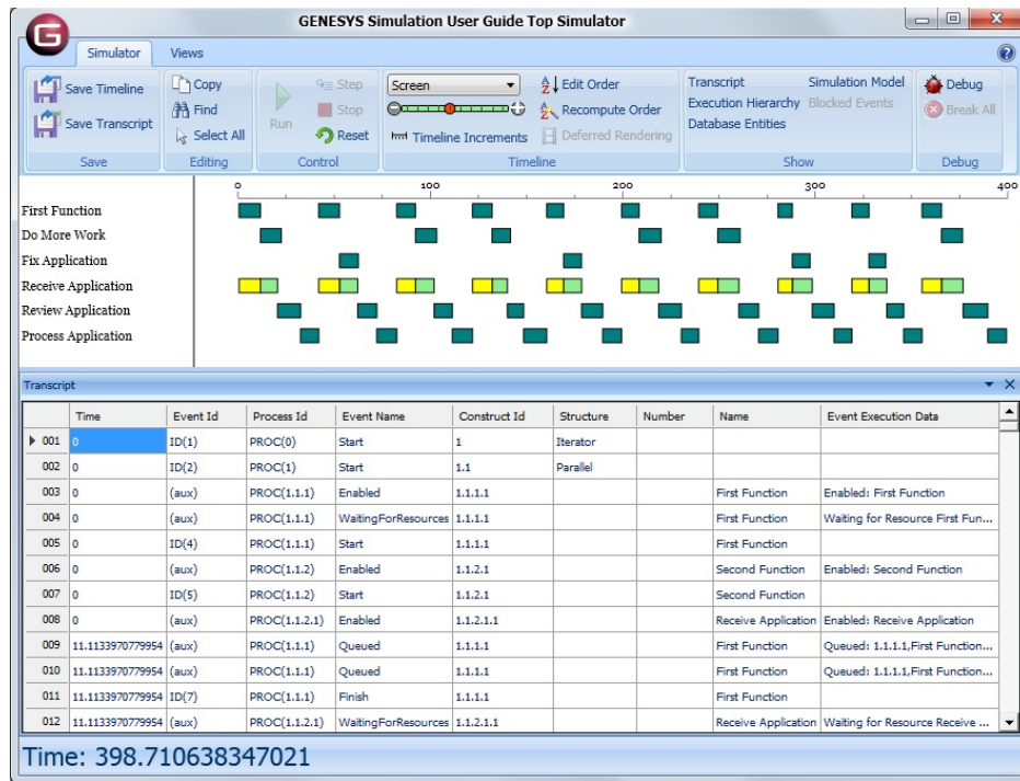
Figure 40 Execute Decomposition Set to False
