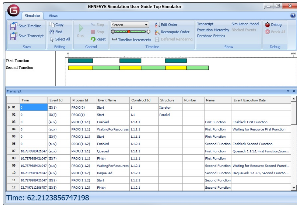
Figure 32 Iterate Construct Simulation Results
