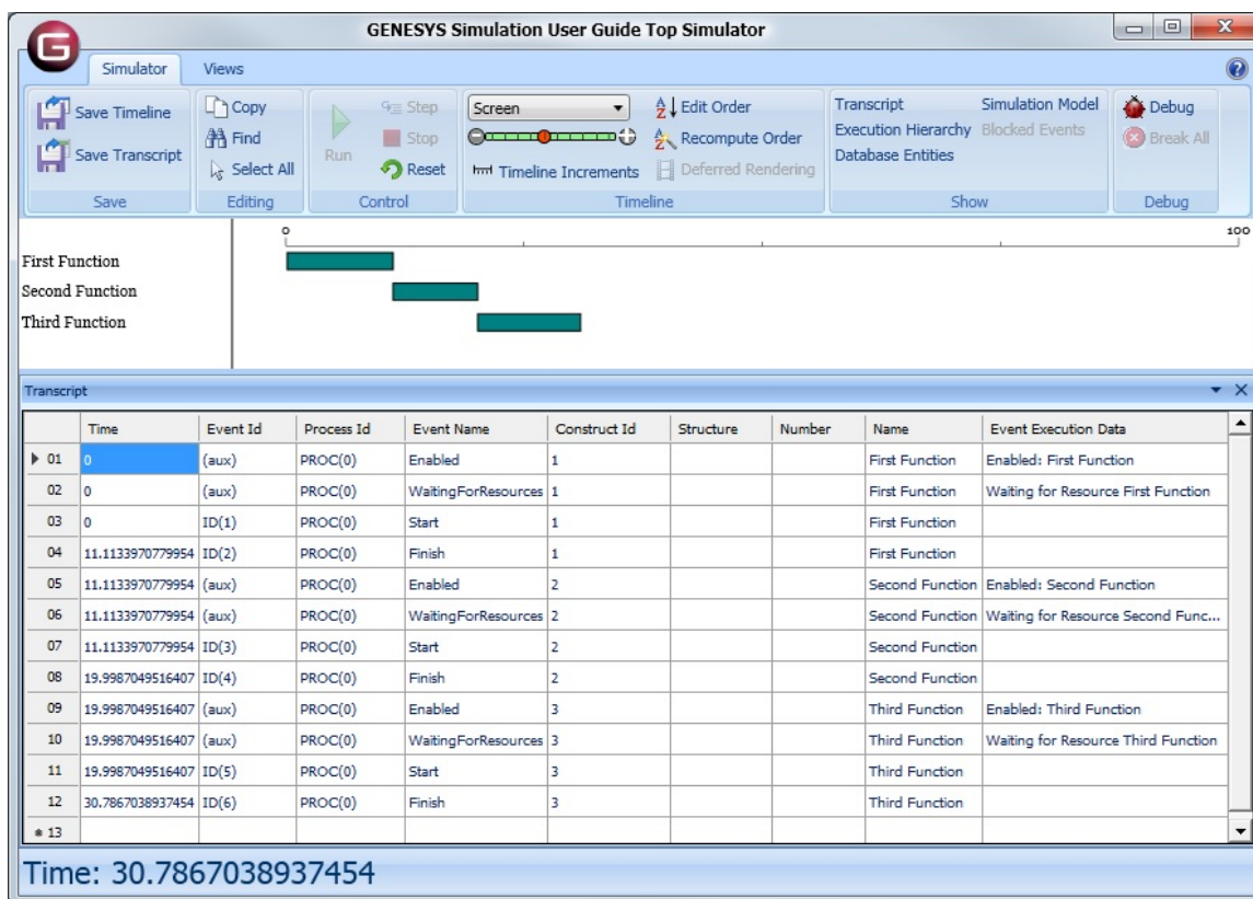
Figure 22 Multiple Functions Simulation Results
