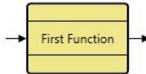
Figure 19 Single Function
