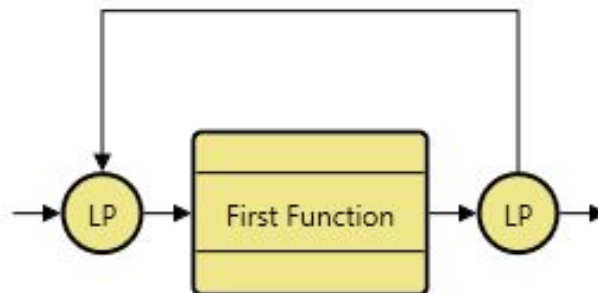
Figure 41 Loop Construct
