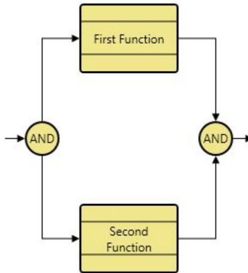
Figure 25 Parallel Construct
