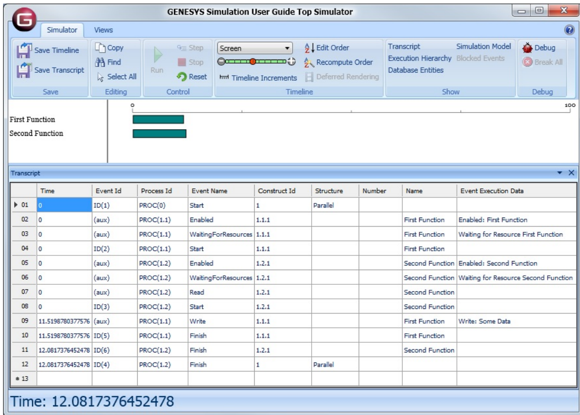
Figure 28 Input Item Simulation Results
