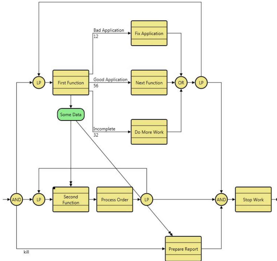
Figure 46 Model with Kill Branch
