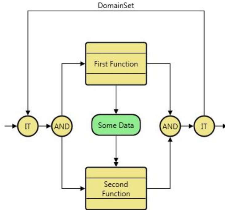
Figure 31 An Iterate Construct
