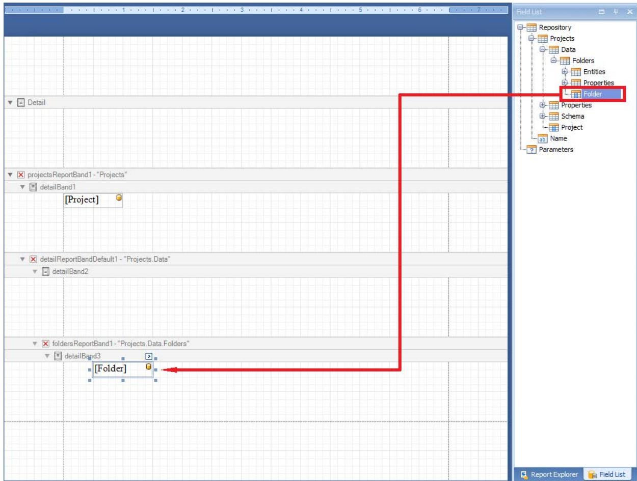
Figure 16: Binding a Label Control to the Folder Object
