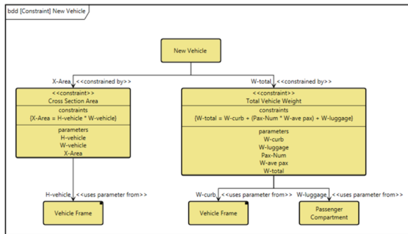
Figure 4 – New Vehicle Constraint bdd
