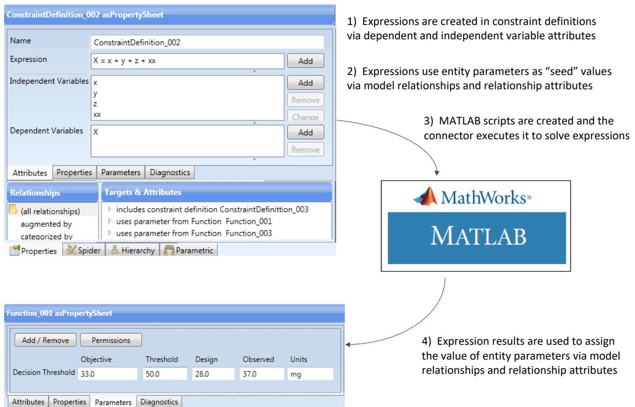
Figure 1 – MATLAB Constraint Solver Concept Graphic
