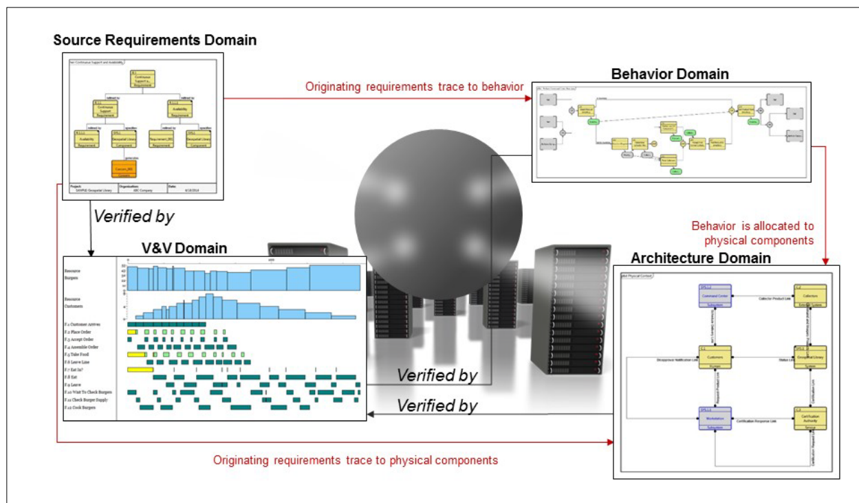
Figure 1 MBSE Activities
