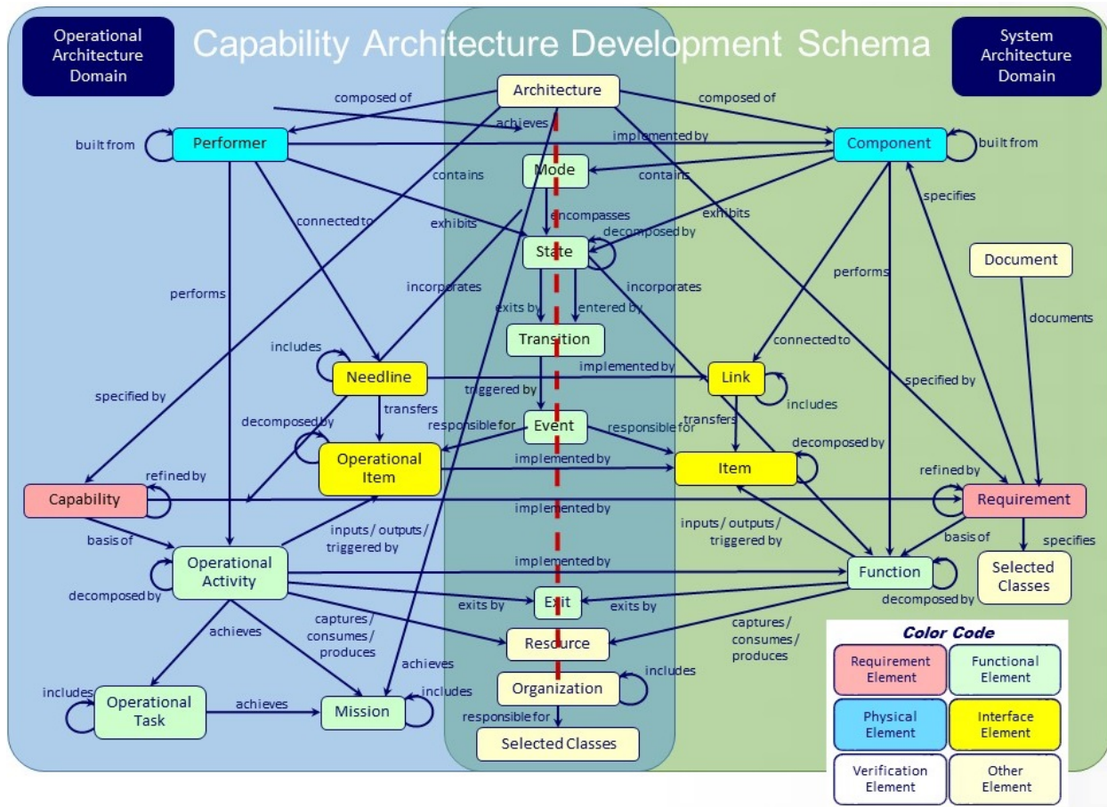
Figure 2 Capability Architecture Development Schema – Key Classes and Relationships of the Schema
